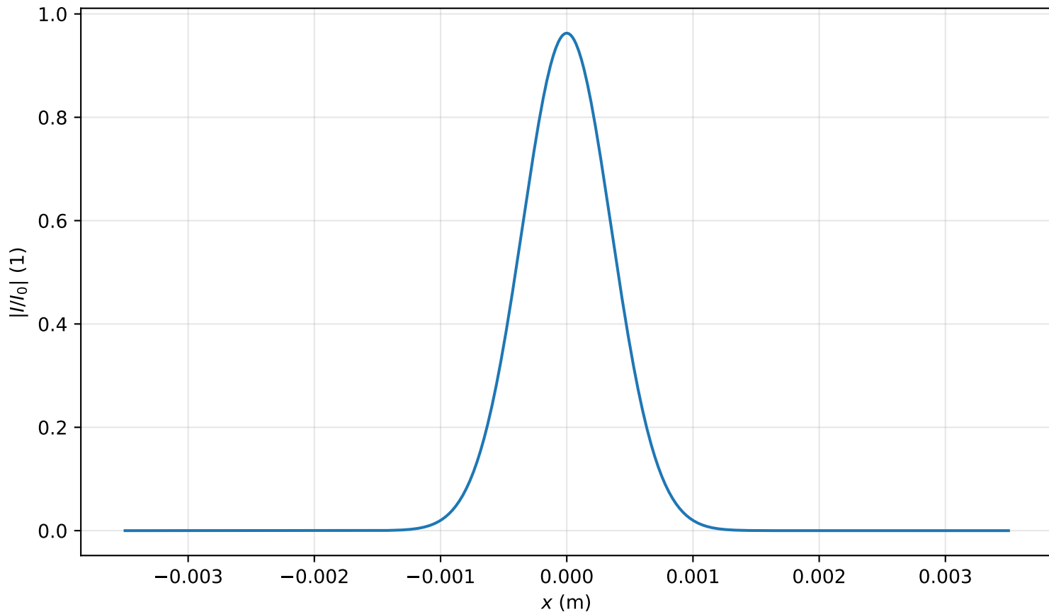
Intensity profile I(x, y = 0, z = 0.478m)/I_0 , P_{in}=0.1P_{cr} , artificial time
